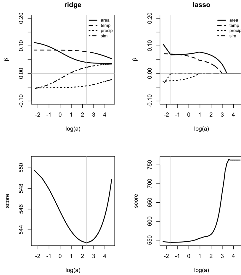
Figure 4.3: Poisson regression coefficient estimate ( \hat{\beta} ) trajectories (top panels) based on the ridge penalty (left panels; b = 2 ) and lasso penalty (right panels; b = 1 ). Regularization score trajectories (bottom panels) based on cross-validation. Vertical gray lines represent the values for the strength parameter a based on the optimal scores.
