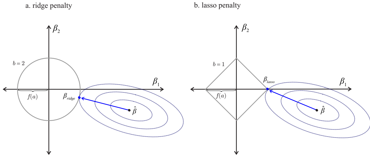
Figure 4.2: Ridge penalty (gray circle, b = 2 ) and lasso penalty (gray diamond, b = 1 ) with three point estimates in parameter space for a model with 2 parameters ( \beta_1, \beta_2 ): the unpenalized estimate ( \hat{\beta} ), the ridge estimate ( \hat{\beta}_{\text{ridge}} ), and the lasso estimate ( \hat{\beta}_{\text{lasso}} ). The arrows indicate the shrinkage induced by the penalty in each case. The ellipses represent contours of the distribution for the unpenalized estimate ( \hat{\beta} ).
